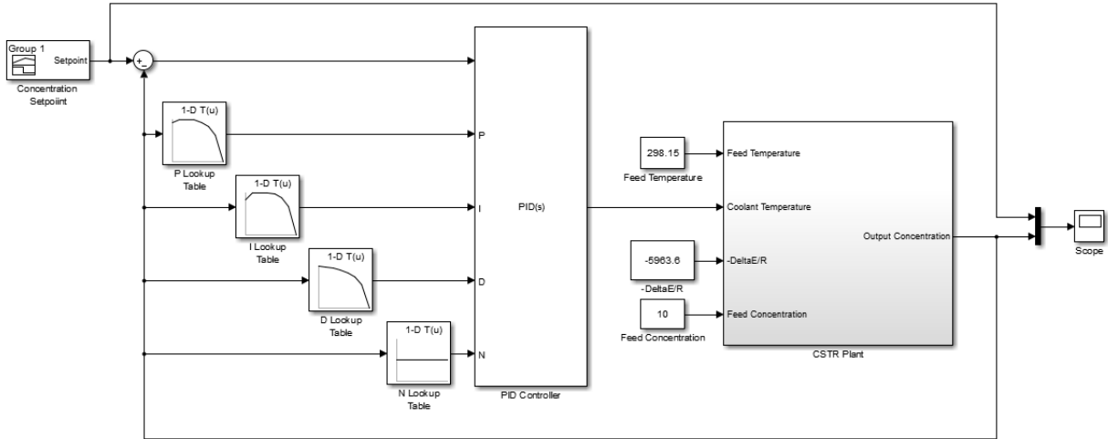
Continuous Stirred Tank Reactor (CSTR) with Gain-Scheduled PID Control
